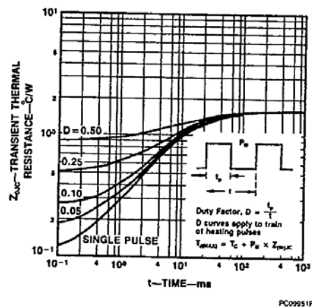
Figure 12 Transient Thermal Resistance vs time for MTP10N08/10N10
